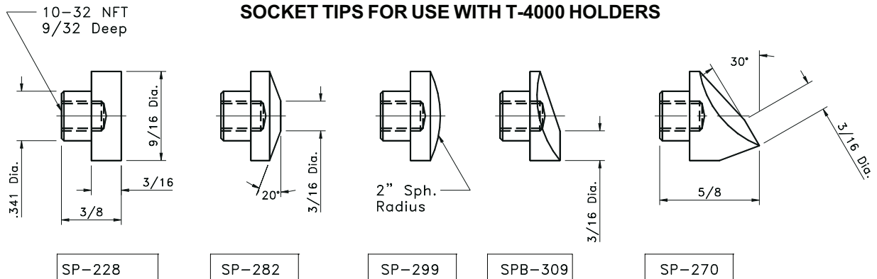
SOCKET TIPS FOR USE WITH T-4000 HOLDERS
