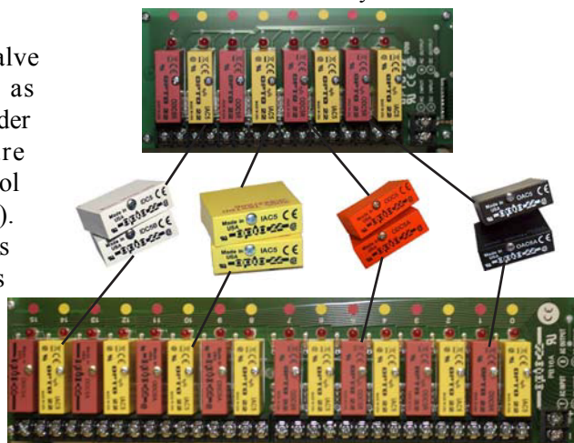
2-8 Welder Interlock Relay Rack Board
