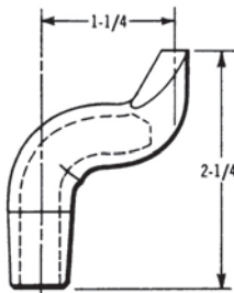
FD-1524-20 FA-2524-20
