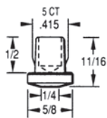
TRUNCATED CONE SE-6332 (Part No. 186-0522)
