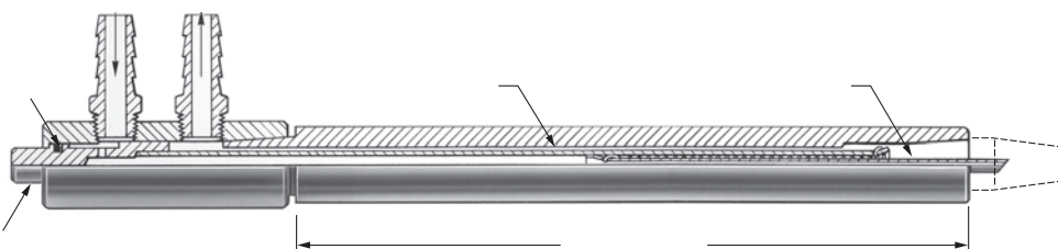
Cross-section of holders with barrels 7/8 inch or less in diameter.
